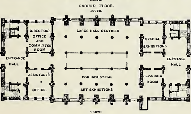
THE FIRST BUILDING IN CENTRAL PARK FLOOR PLANS
